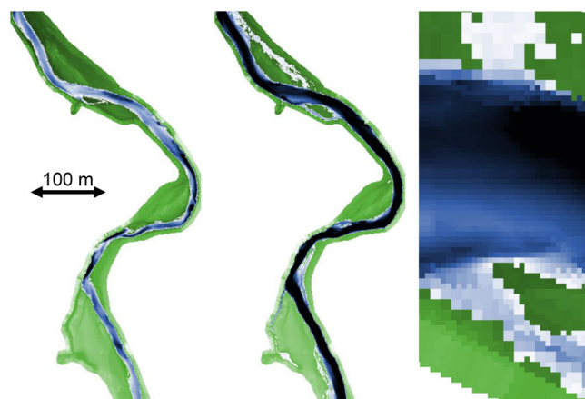
FIGURE 2 Example model representing habitat as a fine grid of square cells. This application uses >108,000 cells that are 1.5 m wide. Cells are shown shaded by depth at a low and high flow (left, center), and a zoom that shows individual cells (right). [Color figure can be viewed at wileyonlinelibrary.com ]
