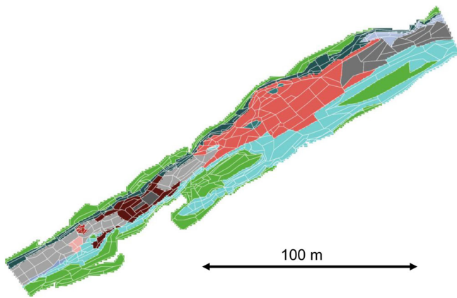
FIGURE 3 Example representation of habitat as dynamic mesohabitat units. Reach-scale habitat variables can include the areas of deep pool habitat (blue), food-producing riffle (red), and shallows suitable for juveniles (light blue). These areas are delineated dynamically from the depth and velocity of hydraulic model cells (outlined in white). Dry cells are green. [Color figure can be viewed at wileyonlinelibrary.com ]
